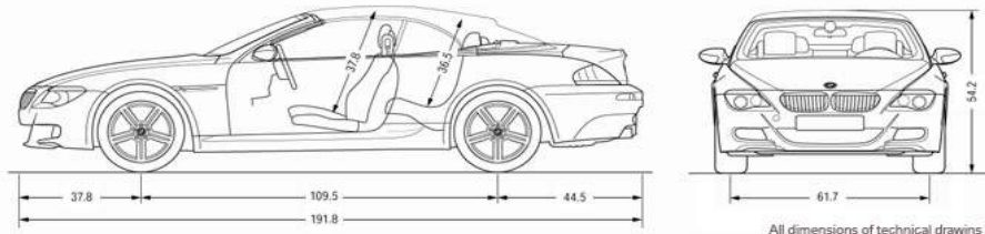
All dimensions of technical drawings in inches.
