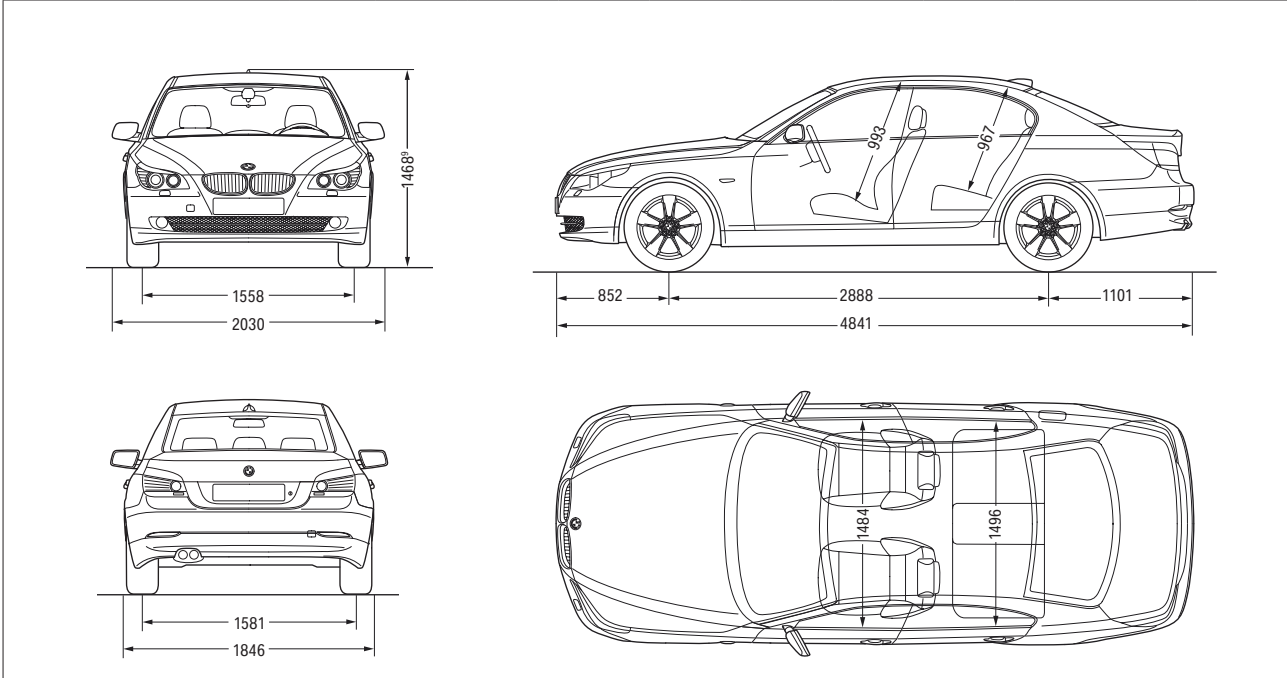
All dimensions in millimetres. Luggage compartment capacity (as per VDA standard): 520 litres (18.4 cu ft).
