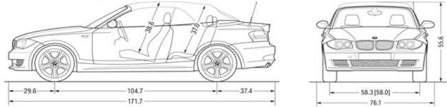
All dimensions are shown in inches, and apply to the 128i with standard wheels. Figure [ ] refer to 135i.
